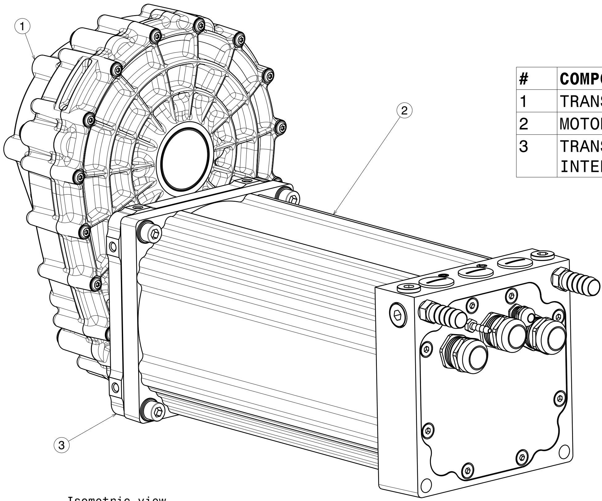
Isometric view Scale: 1:2
